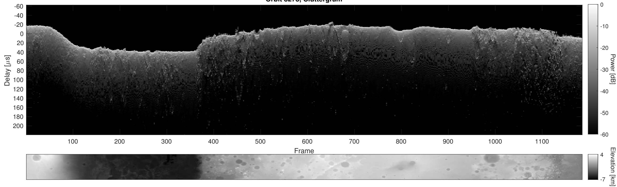
Orbit 8278, Cluttergram
