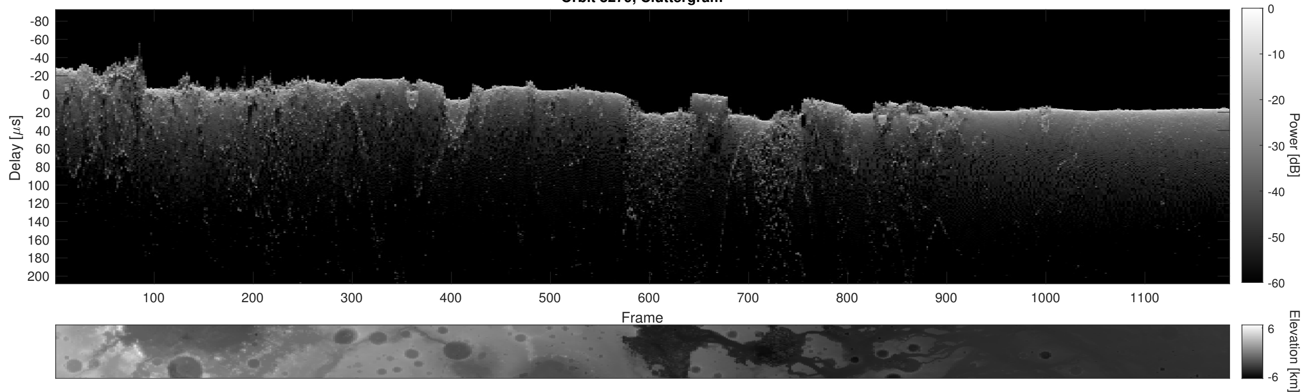
Orbit 8279, Cluttergram
