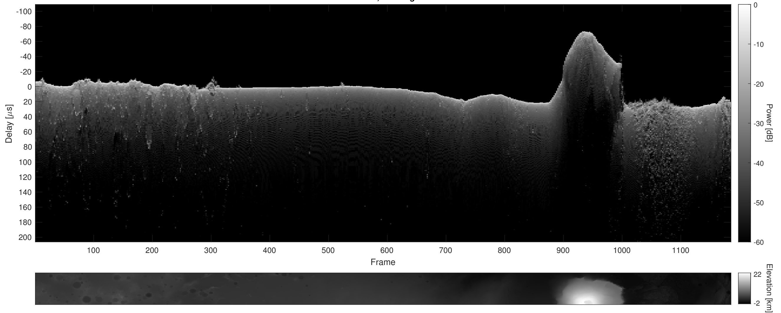
Orbit 8280, Cluttergram
