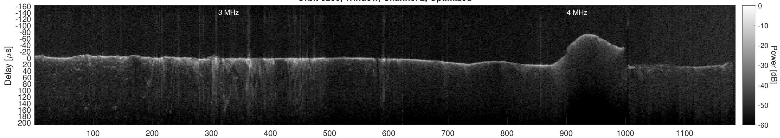
Orbit 8280, Cluttergram
