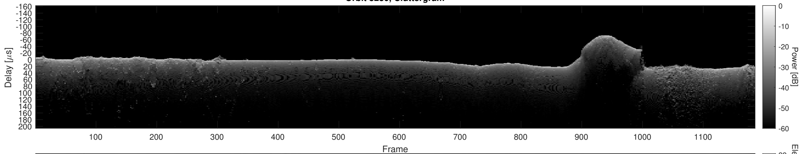
Orbit 8280, Cluttergram
