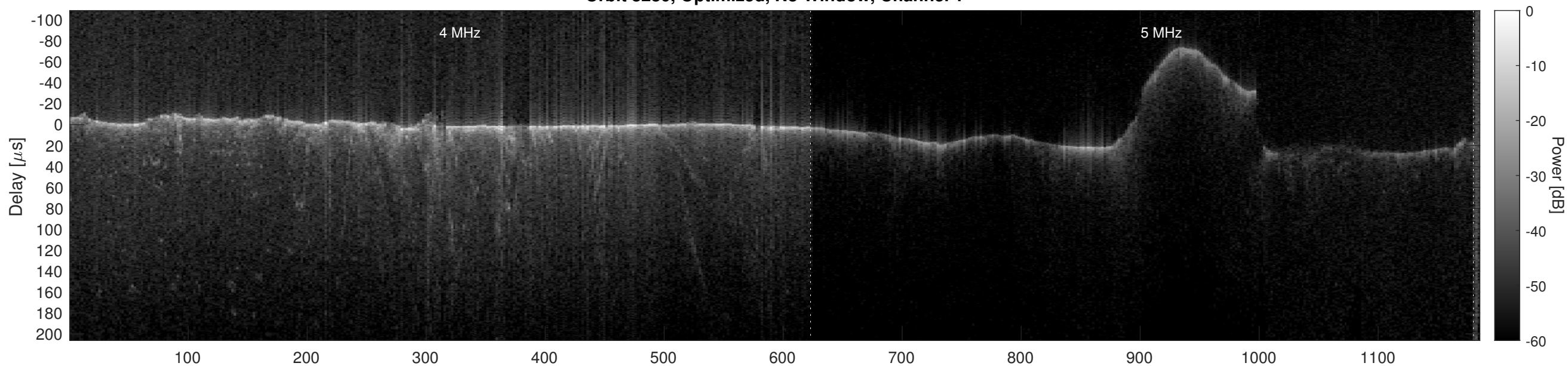
Orbit 8280, Optimized, No Window, Channel 2
