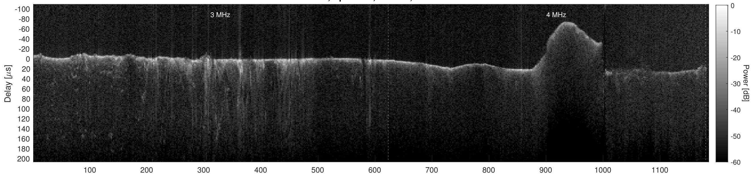
Orbit 8280, Cluttergram
