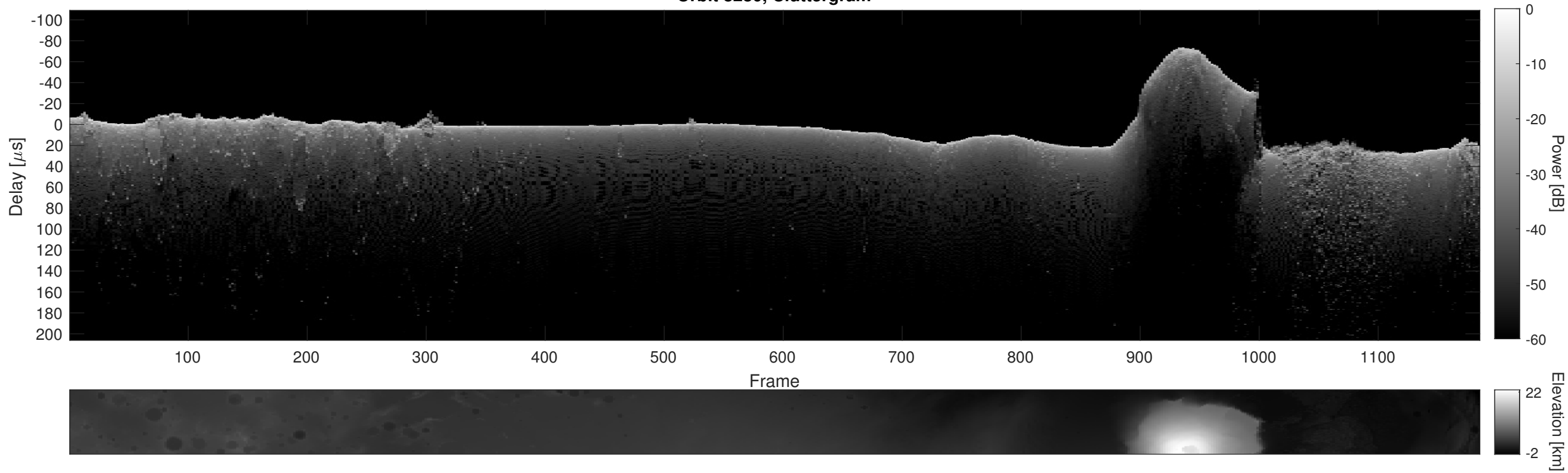
Orbit 8280, Cluttergram
