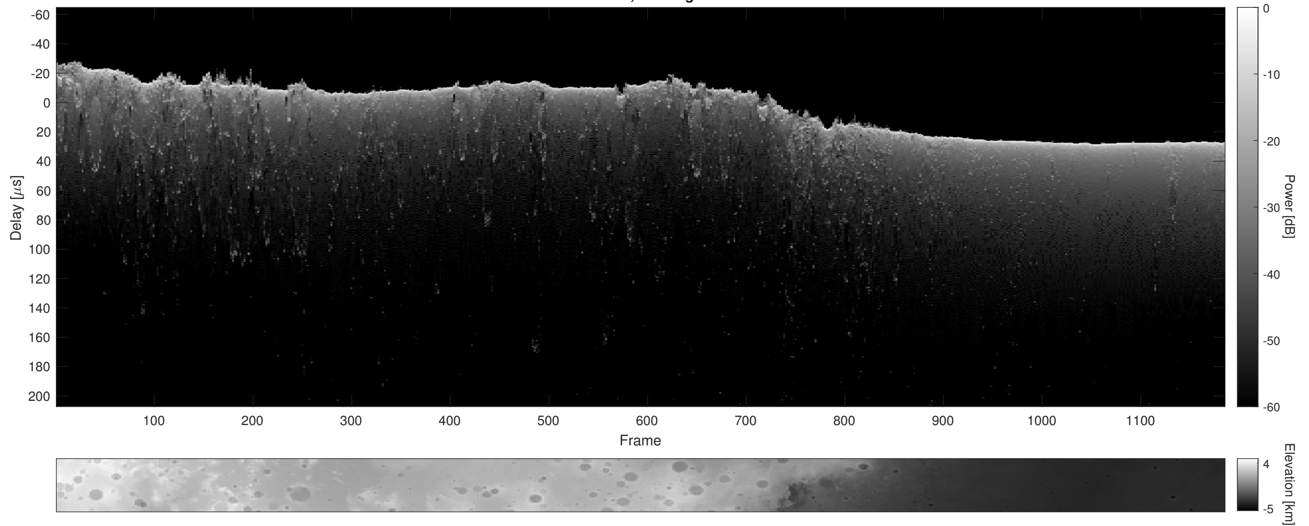
Orbit 8281, Cluttergram
