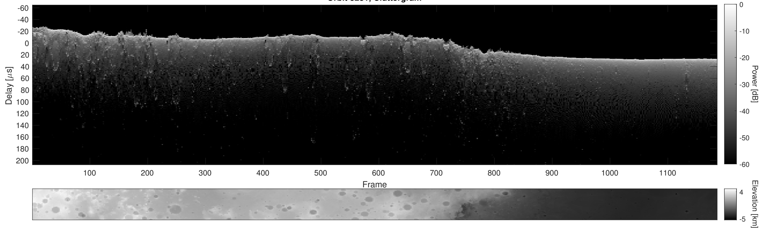
Orbit 8281, Cluttergram
