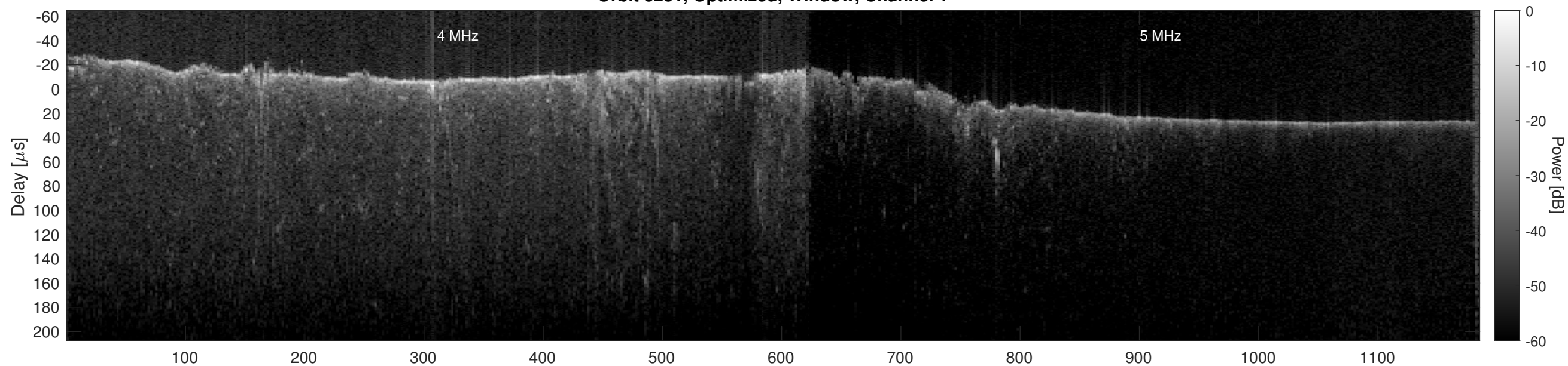
Orbit 8281, Optimized, Window, Channel 2
