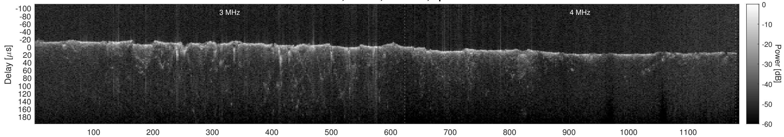
Orbit 8282, Cluttergram
