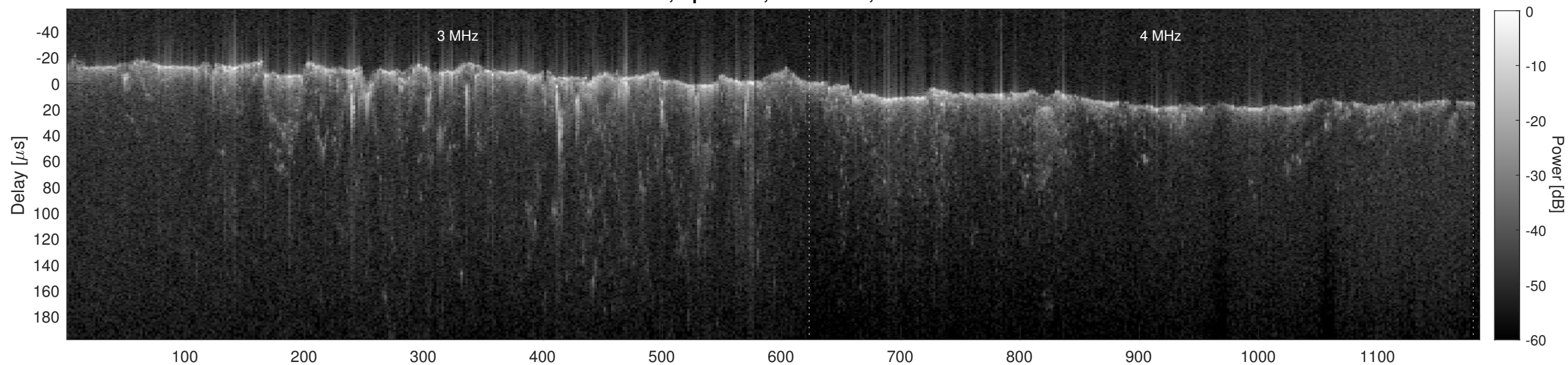
Orbit 8282, Cluttergram
