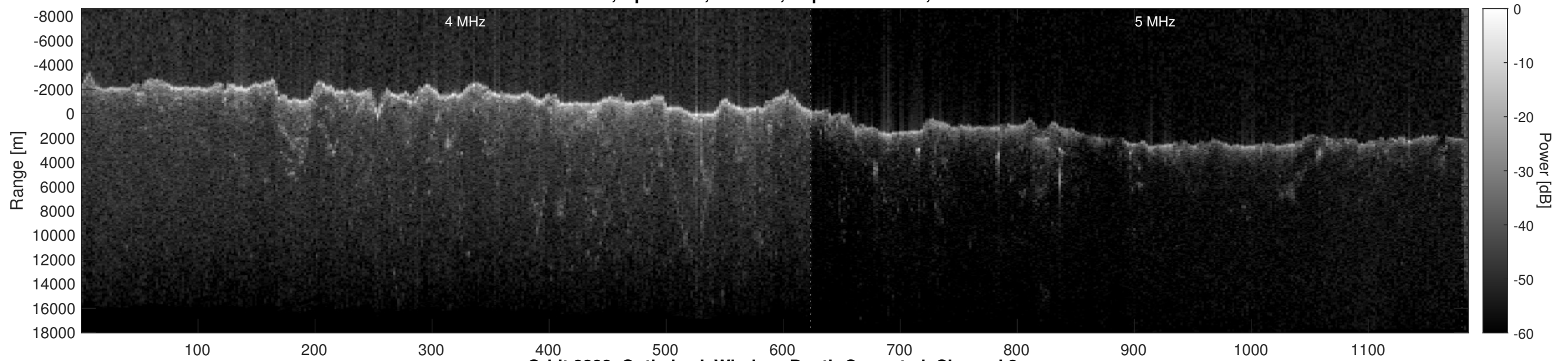
Orbit 8282, Optimized, Window, Depth-Corrected, Channel 2
