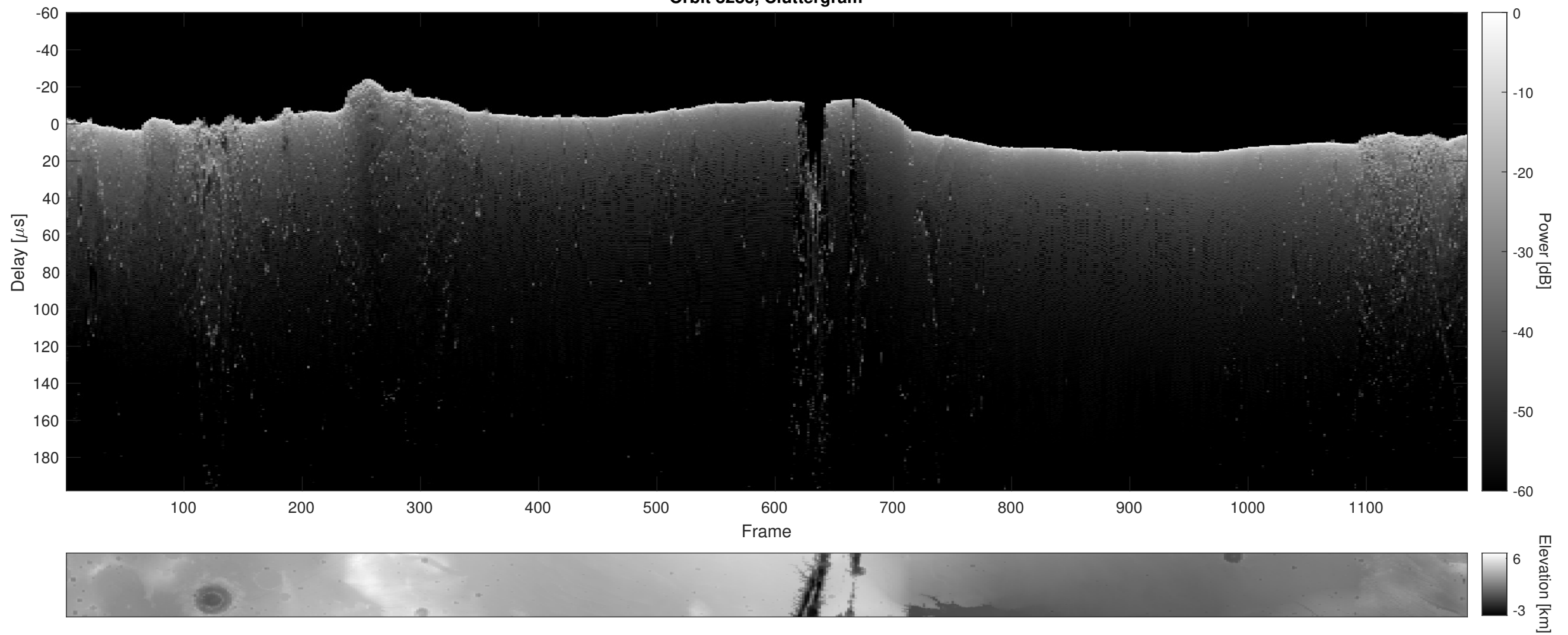
Orbit 8283, Cluttergram
