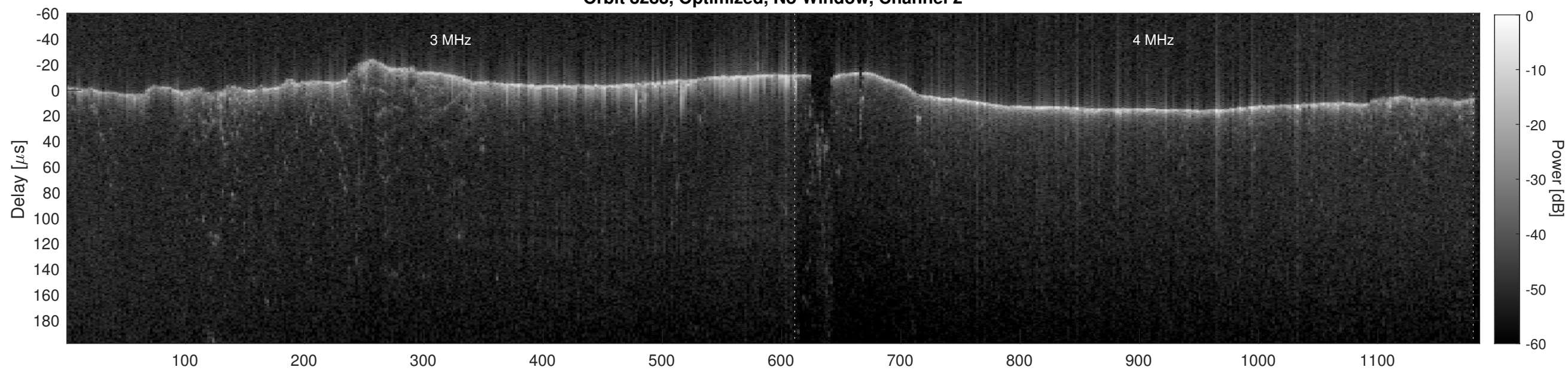
Orbit 8283, Cluttergram
