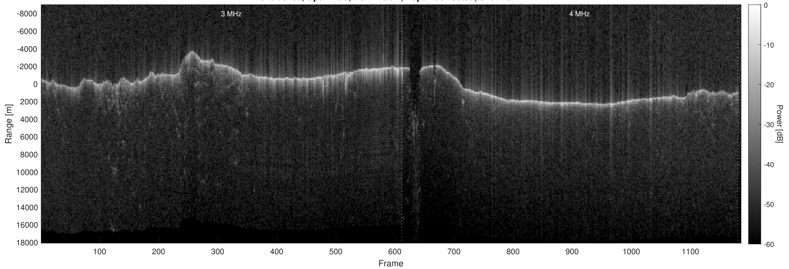
Orbit 8283, Optimized, No Window, Depth-Corrected, Channel 2
