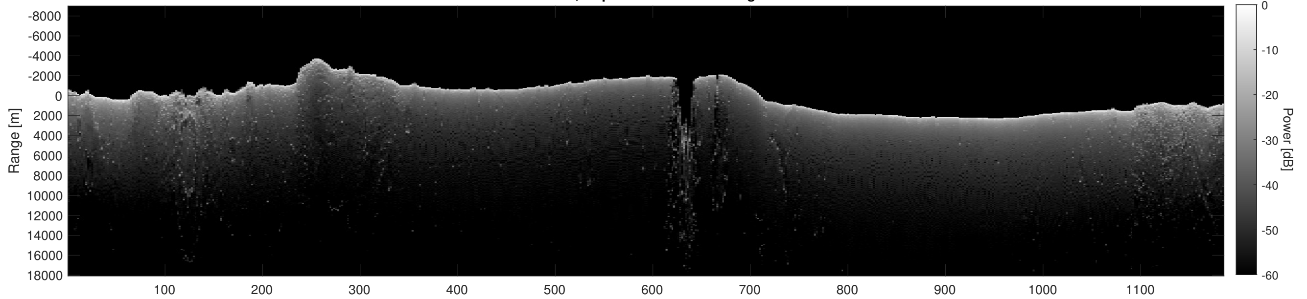
Orbit 8283, Depth-Corrected Cluttergram
