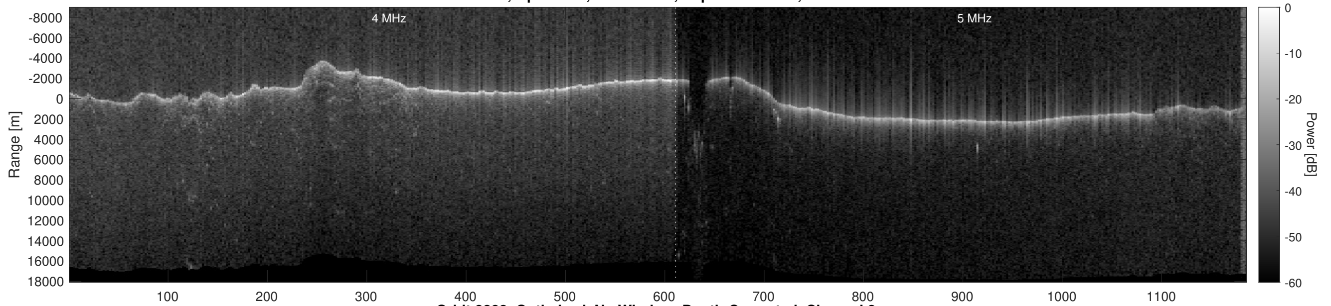
Orbit 8283, Optimized, No Window, Depth-Corrected, Channel 2
