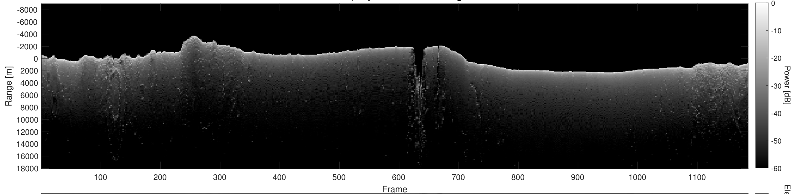
Orbit 8283, Depth-Corrected Cluttergram
