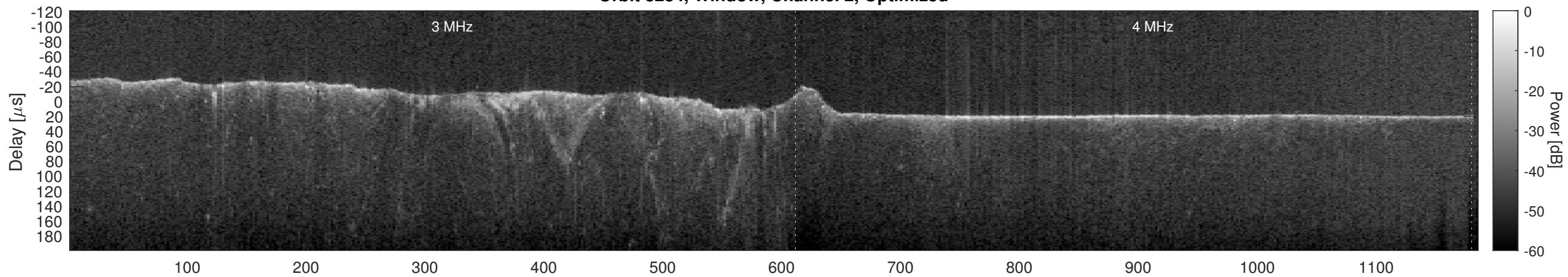
Orbit 8284, Cluttergram
