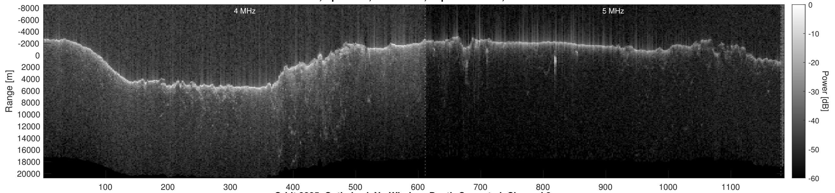
Orbit 8285, Optimized, No Window, Depth-Corrected, Channel 2
