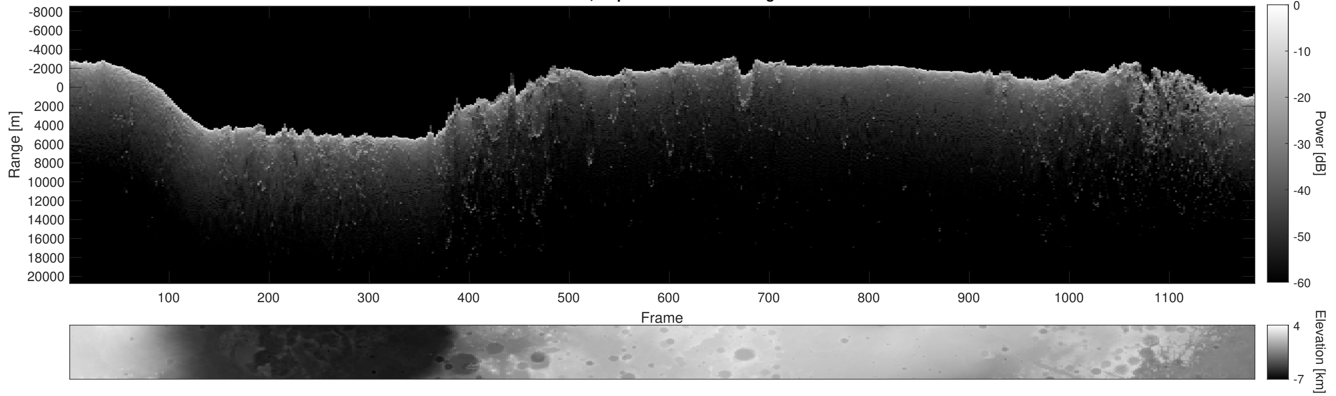
Orbit 8285, Depth-Corrected Cluttergram
