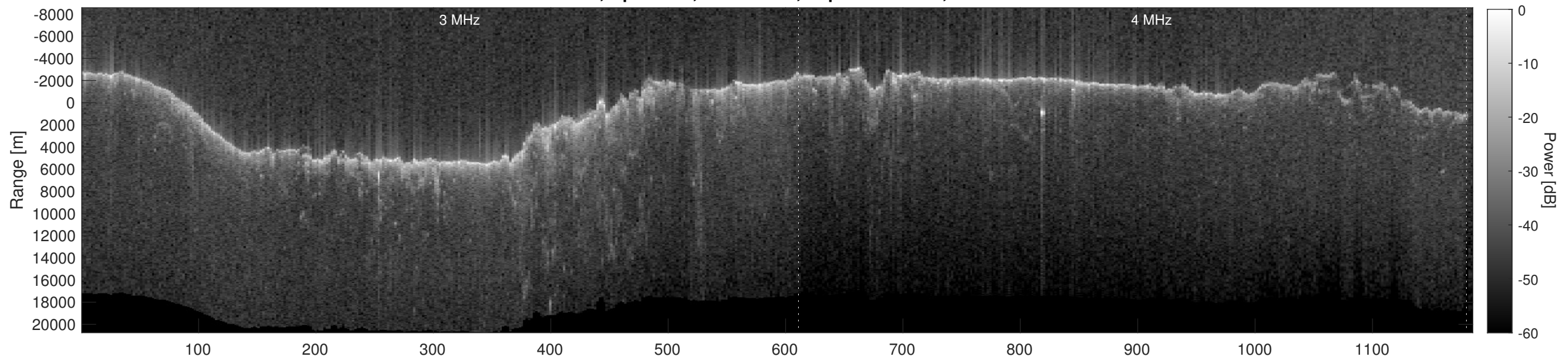
Orbit 8285, Depth-Corrected Cluttergram
