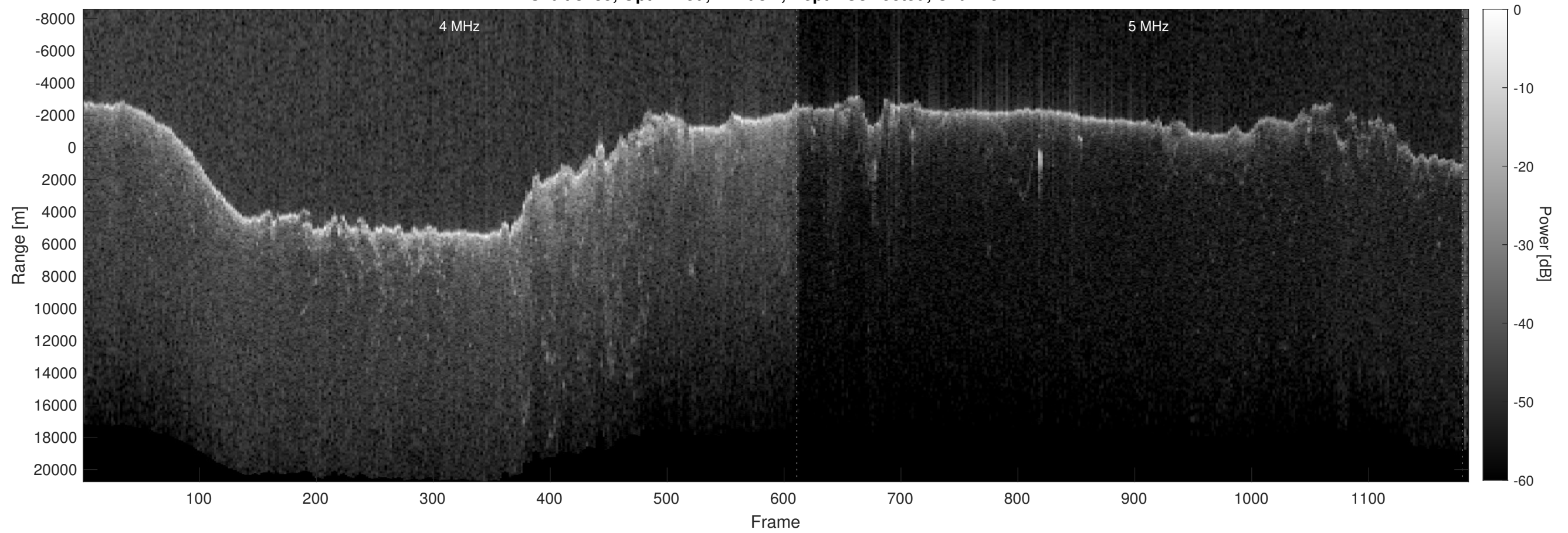
Orbit 8285, Optimized, Window, Depth-Corrected, Channel 2
