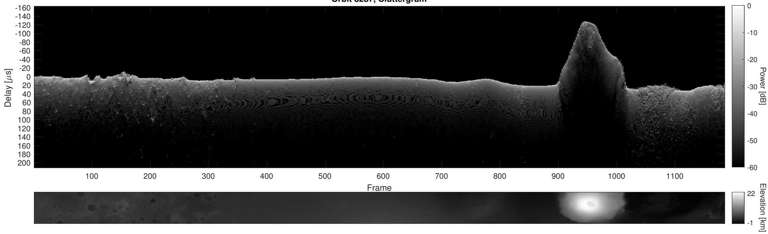
Orbit 8287, Cluttergram
