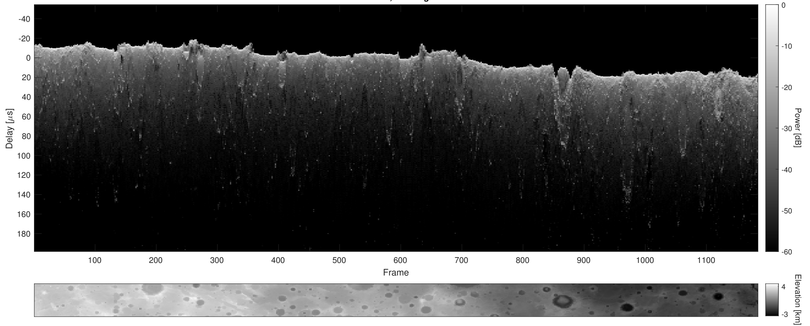
Orbit 8289, Cluttergram
