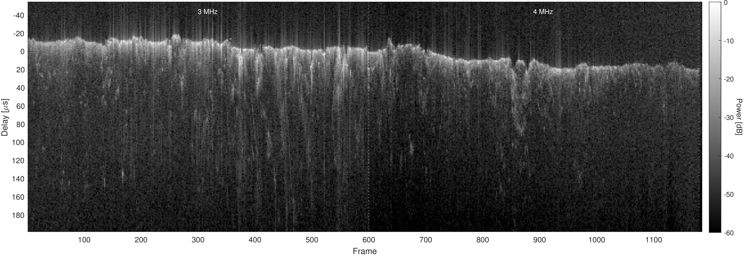
Orbit 8289, Optimized, No Window, Channel 2
