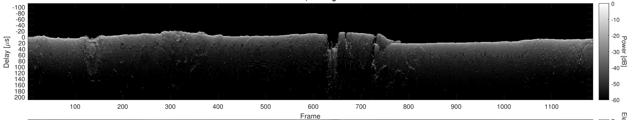
Orbit 8290, Cluttergram
