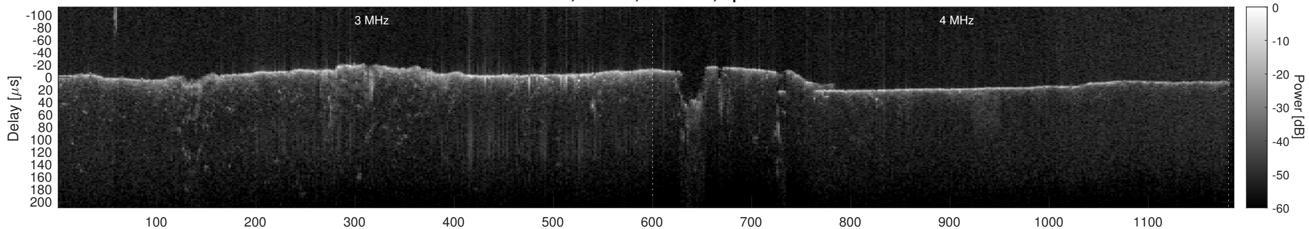
Orbit 8290, Cluttergram
