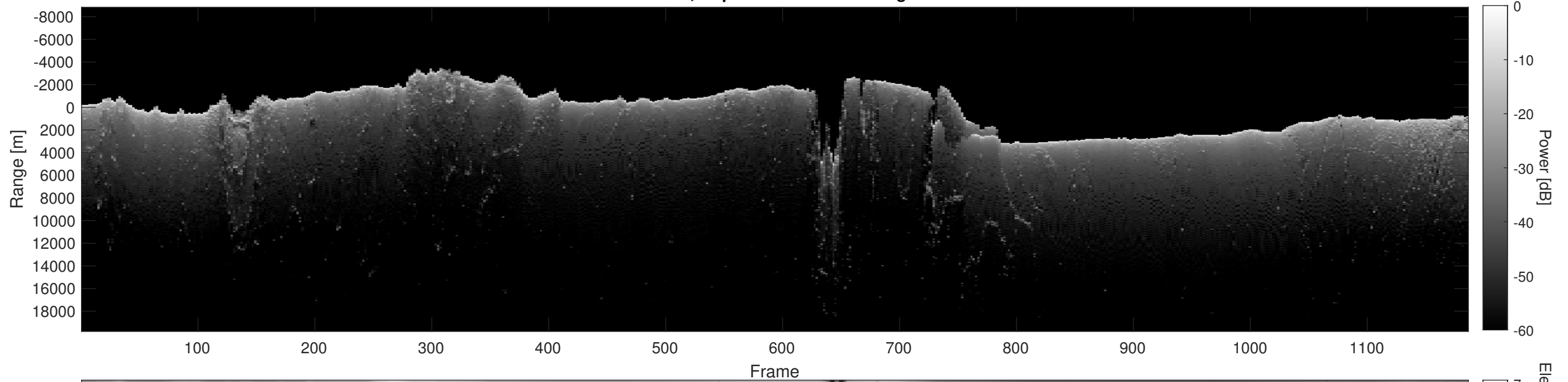
Orbit 8290, Depth-Corrected Cluttergram
