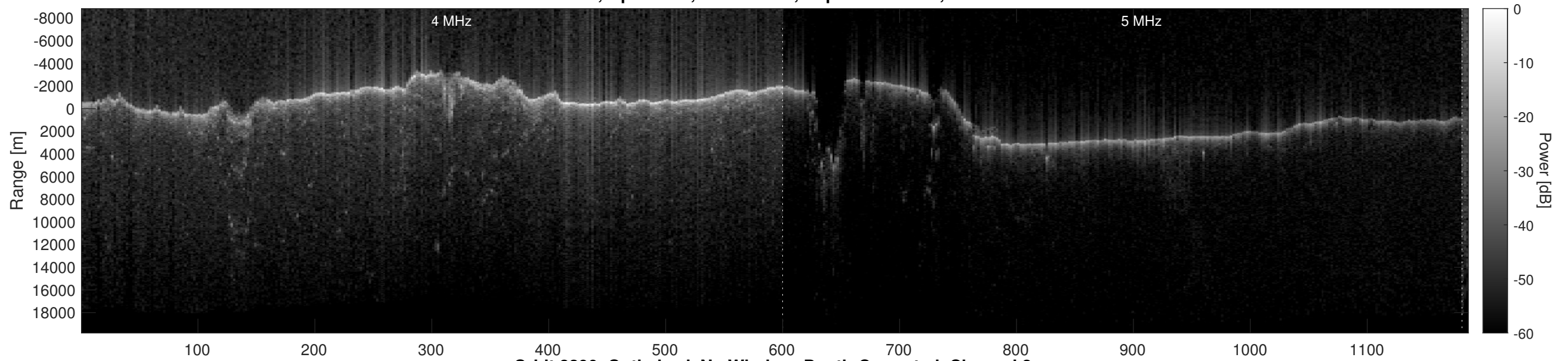
Orbit 8290, Optimized, No Window, Depth-Corrected, Channel 2
