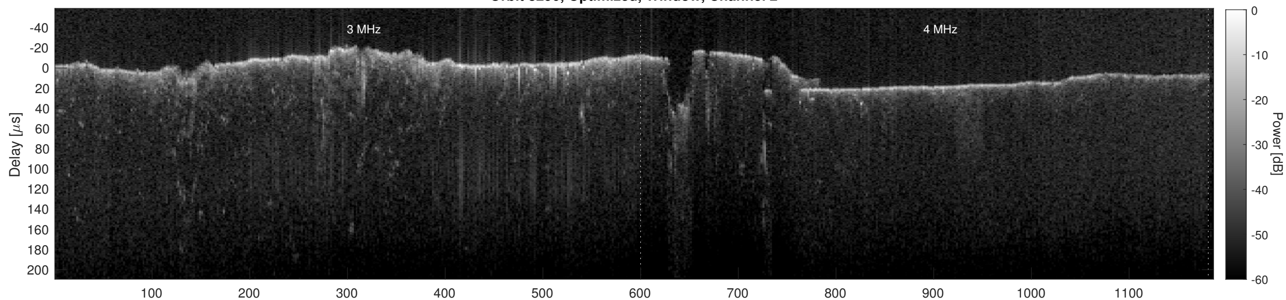
Orbit 8290, Cluttergram
