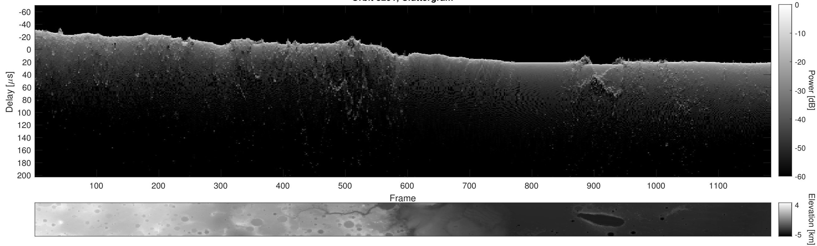
Orbit 8291, Cluttergram
