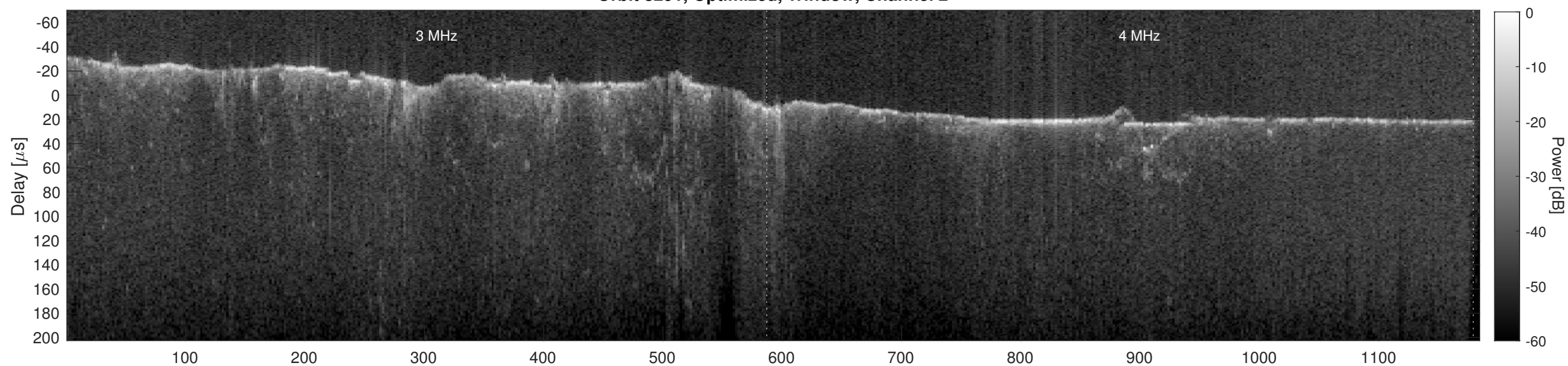
Orbit 8291, Cluttergram
