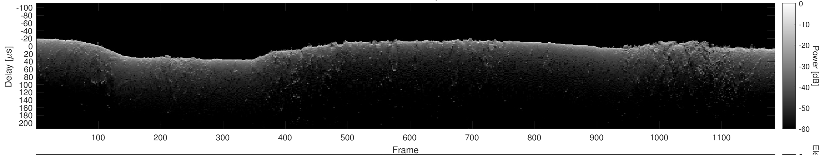
Orbit 8292, Cluttergram
