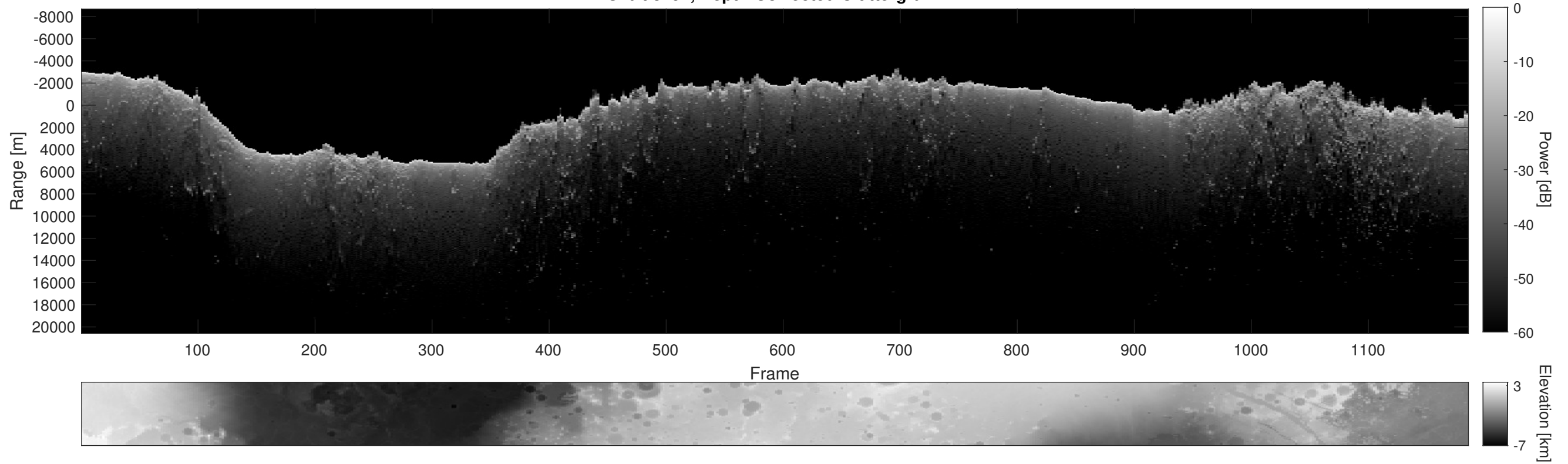
Orbit 8292, Depth-Corrected Cluttergram
