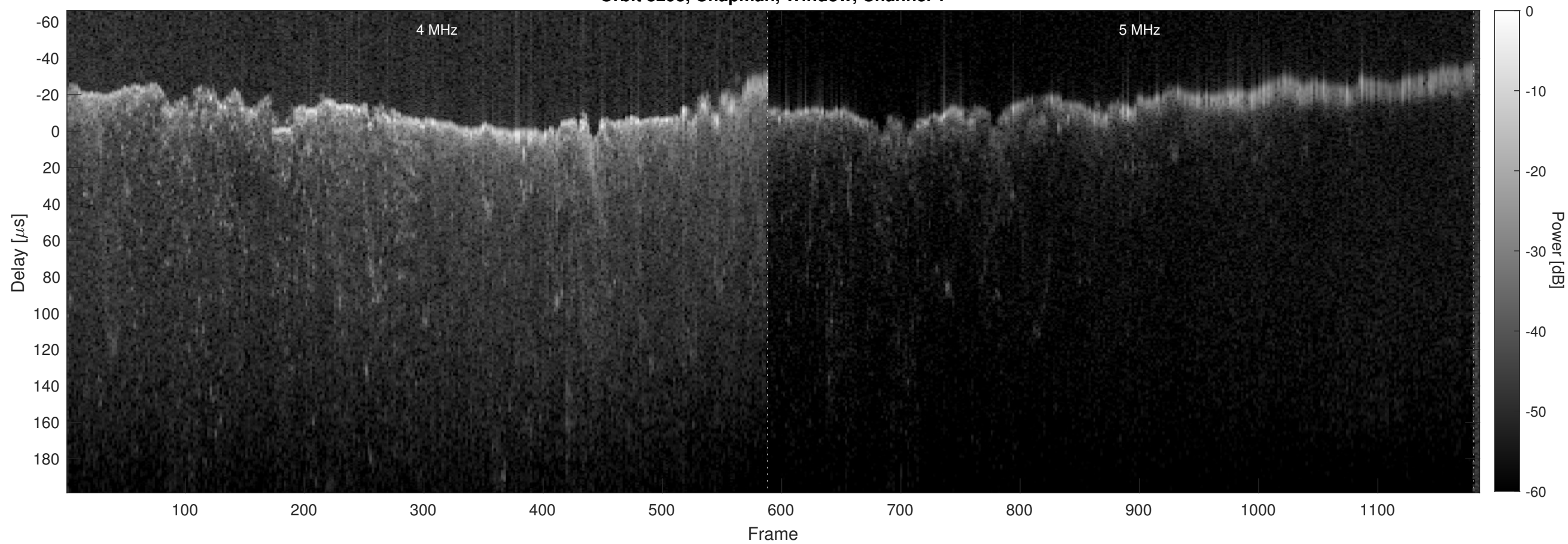
Orbit 8293, Chapman, Window, Channel 2
