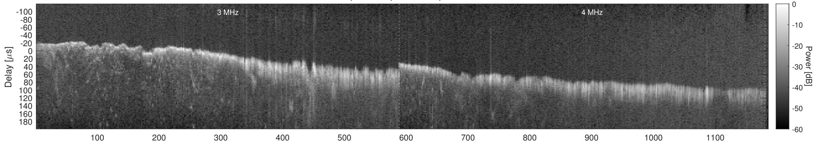
Orbit 8293, Window, Channel 2, Chapman
