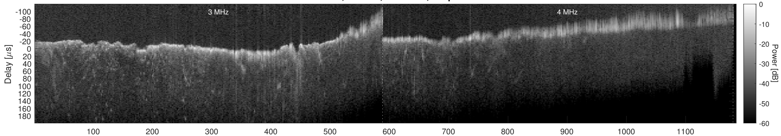
Orbit 8293, Window, Channel 2, Optimized
