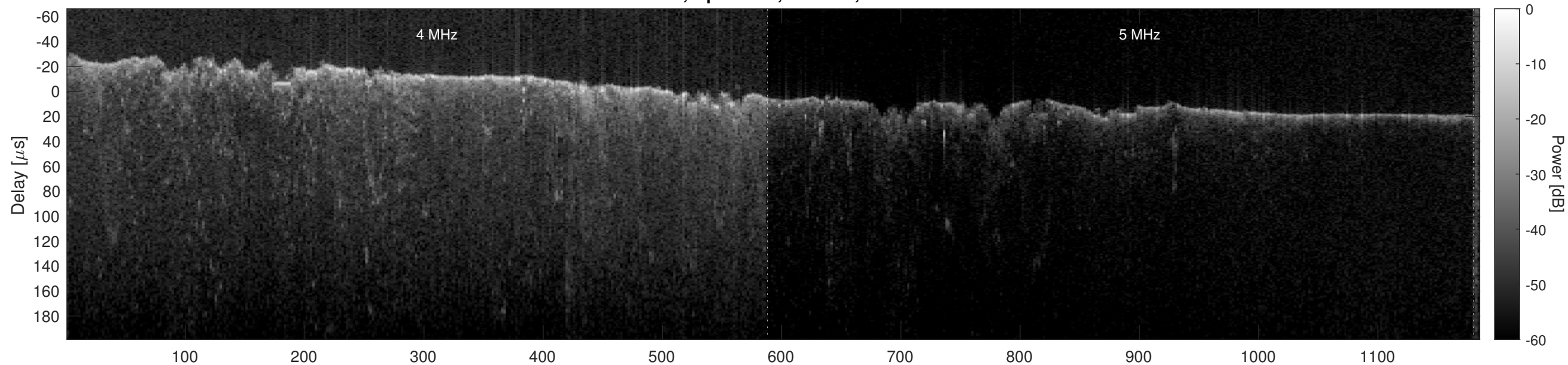
Orbit 8293, Optimized, Window, Channel 2
