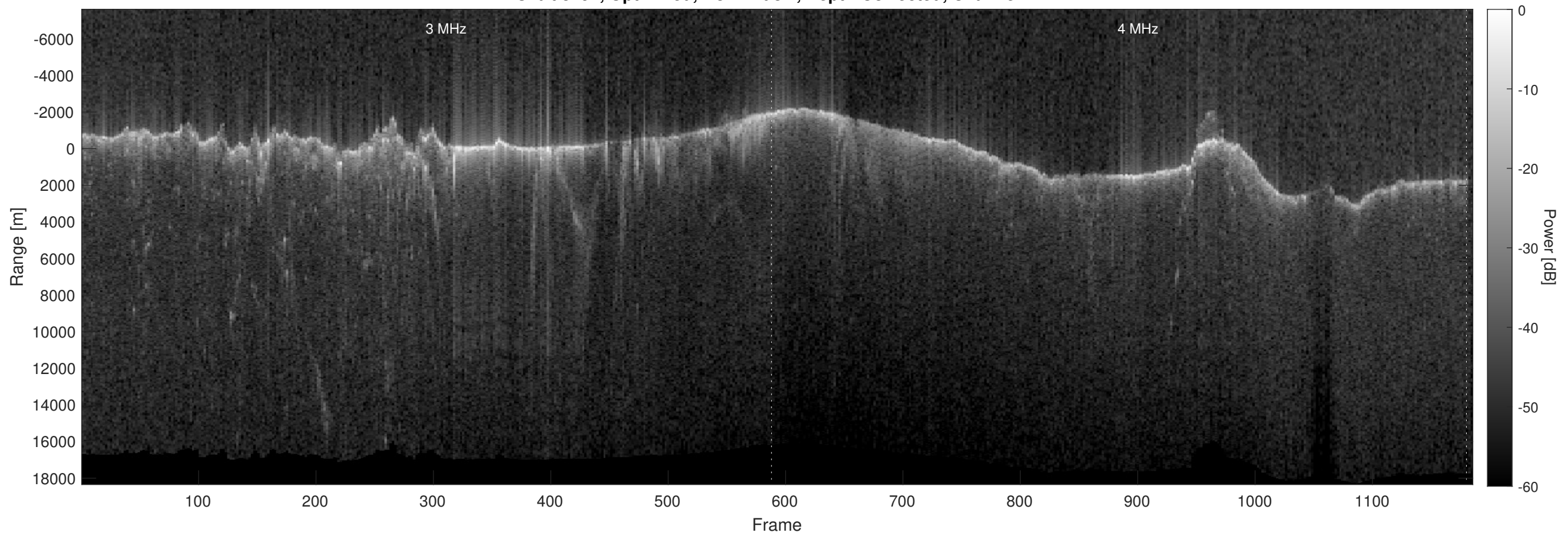
Orbit 8294, Optimized, No Window, Depth-Corrected, Channel 2
