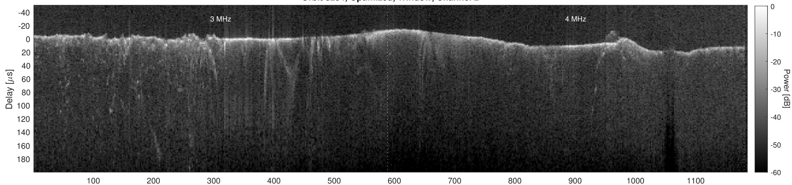
Orbit 8294, Cluttergram
