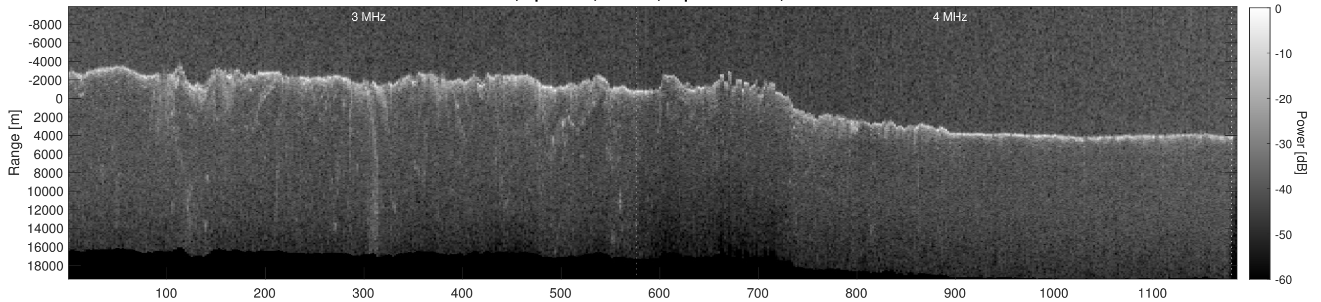
Orbit 8295, Depth-Corrected Cluttergram
