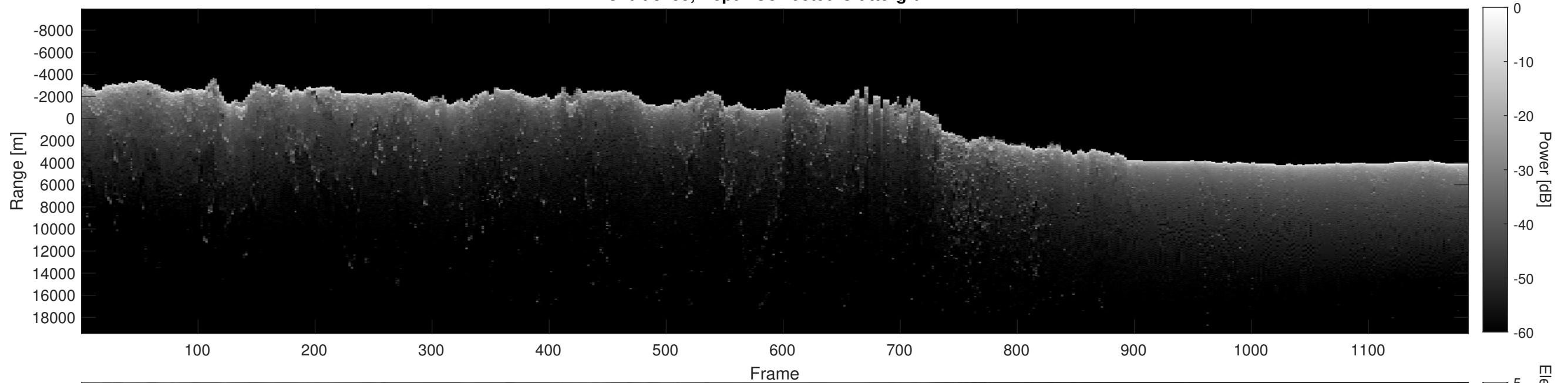
Orbit 8295, Depth-Corrected Cluttergram
