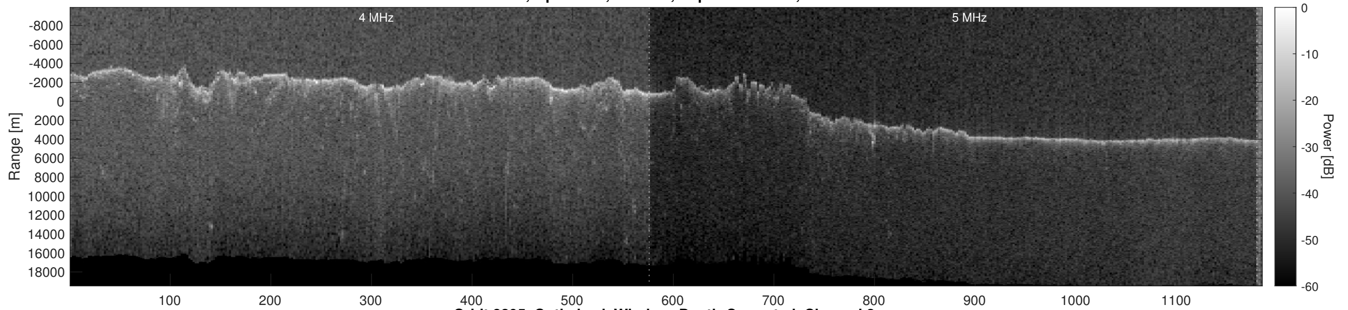
Orbit 8295, Optimized, Window, Depth-Corrected, Channel 2
