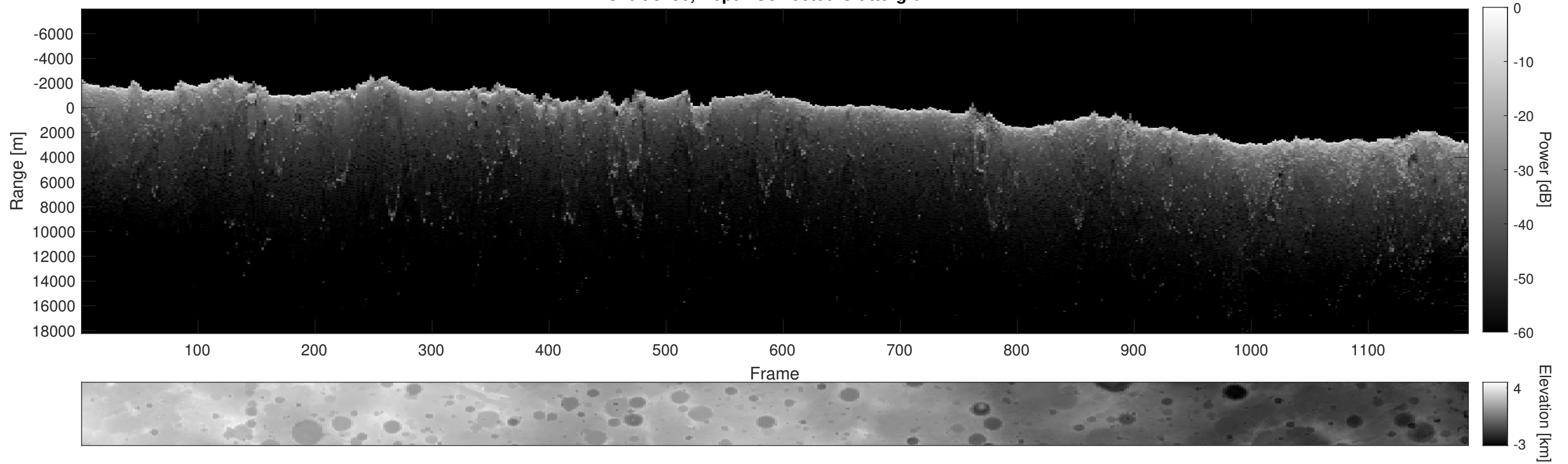
Orbit 8296, Depth-Corrected Cluttergram
