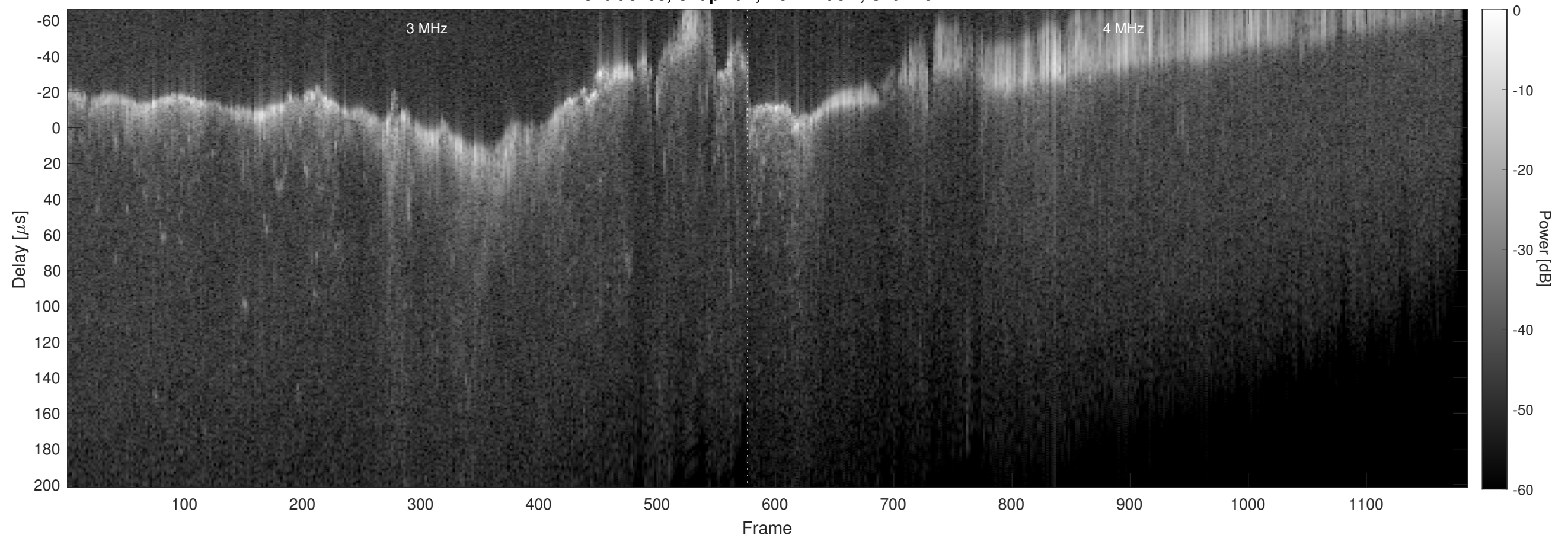
Orbit 8298, Chapman, No Window, Channel 2
