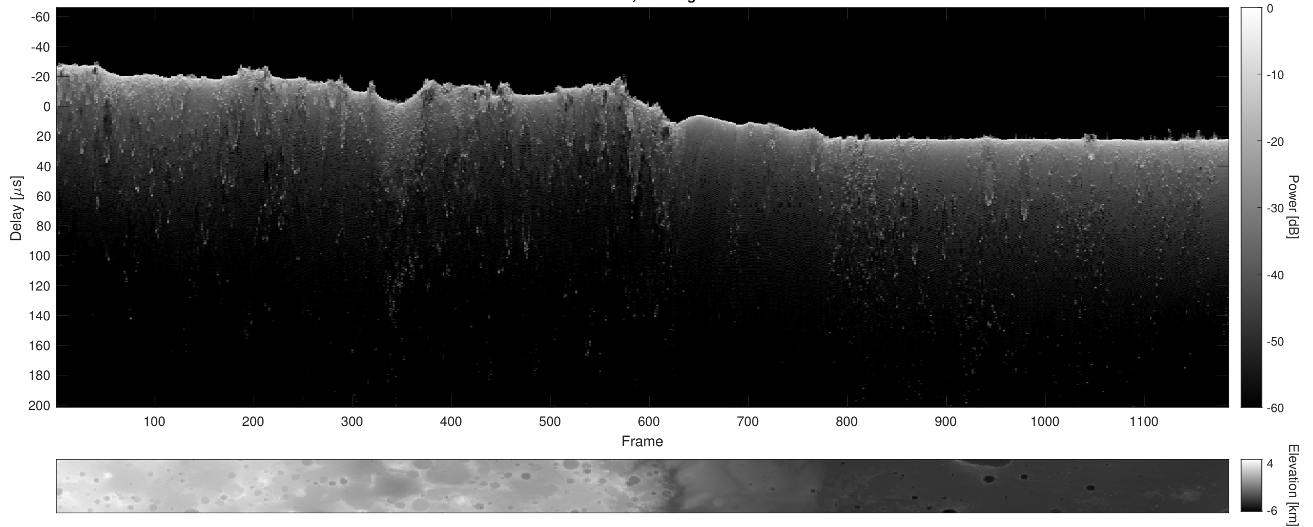
Orbit 8298, Cluttergram
