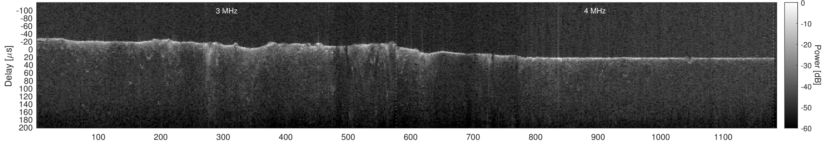
Orbit 8298, Cluttergram
