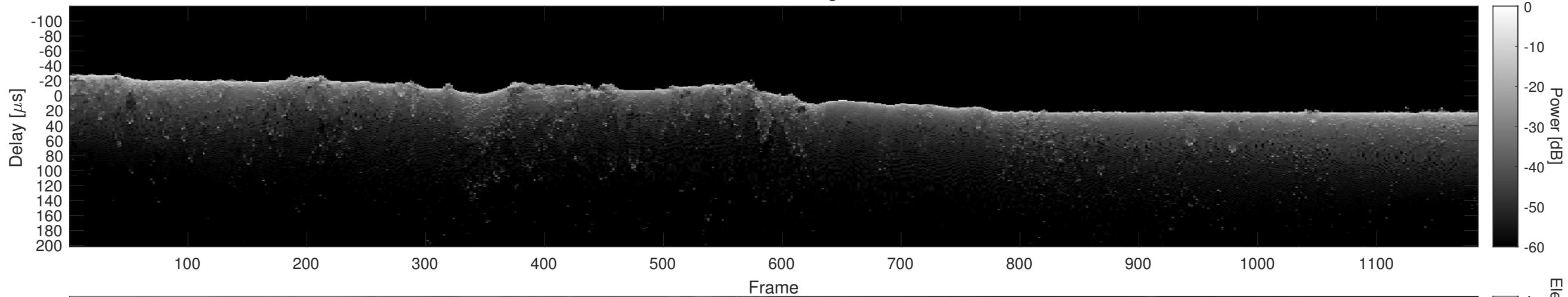
Orbit 8298, Cluttergram
