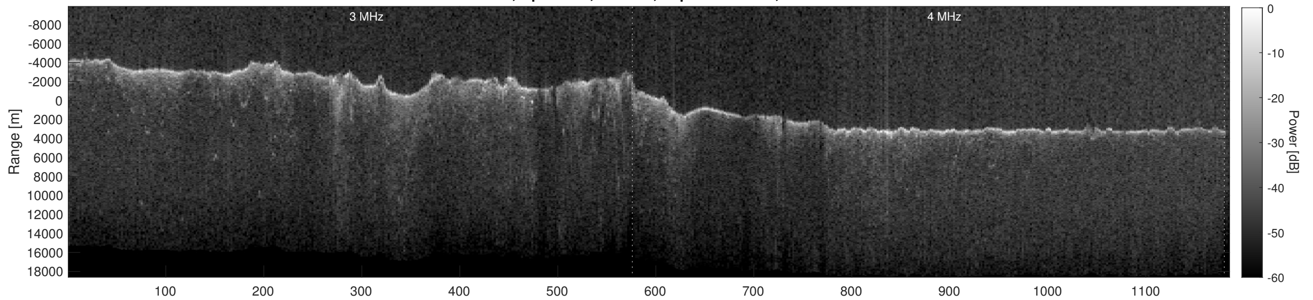
Orbit 8298, Depth-Corrected Cluttergram
