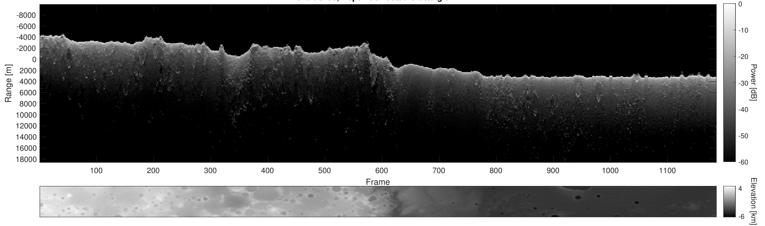
Orbit 8298, Depth-Corrected Cluttergram
