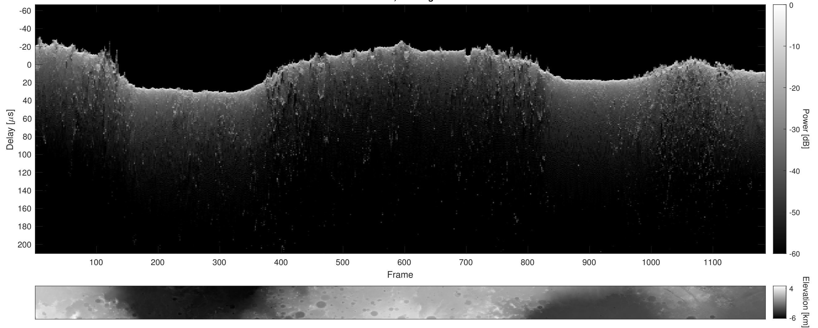
Orbit 8299, Cluttergram
