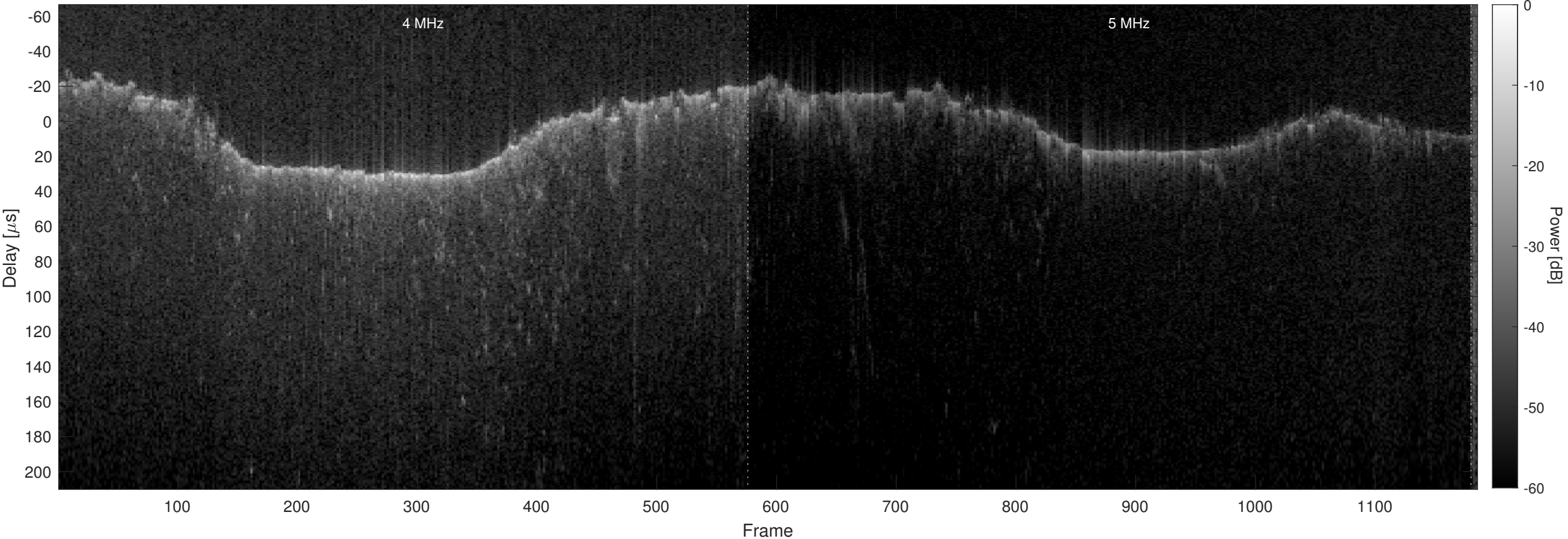
Orbit 8299, Optimized, No Window, Channel 2
