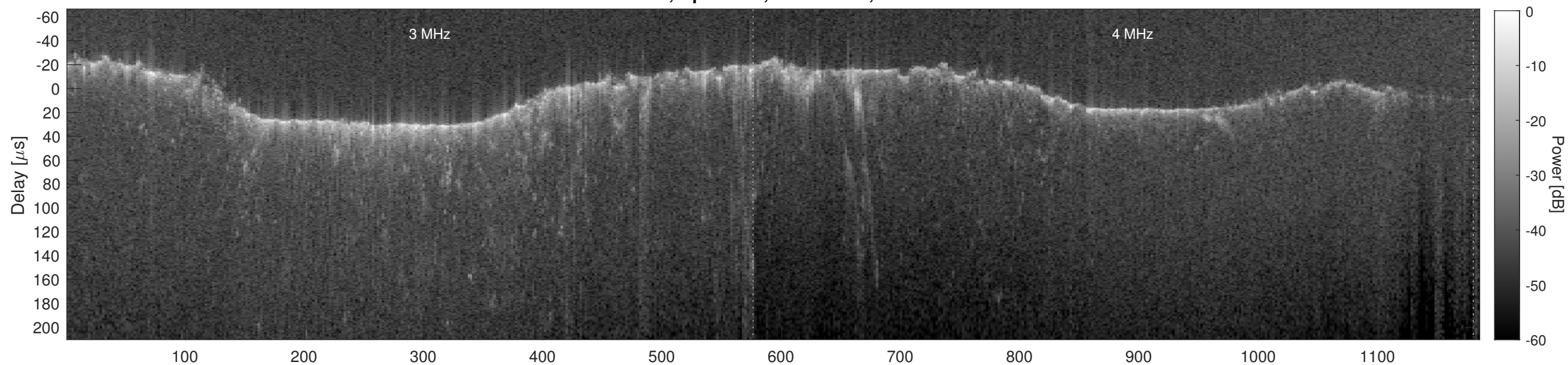
Orbit 8299, Cluttergram
