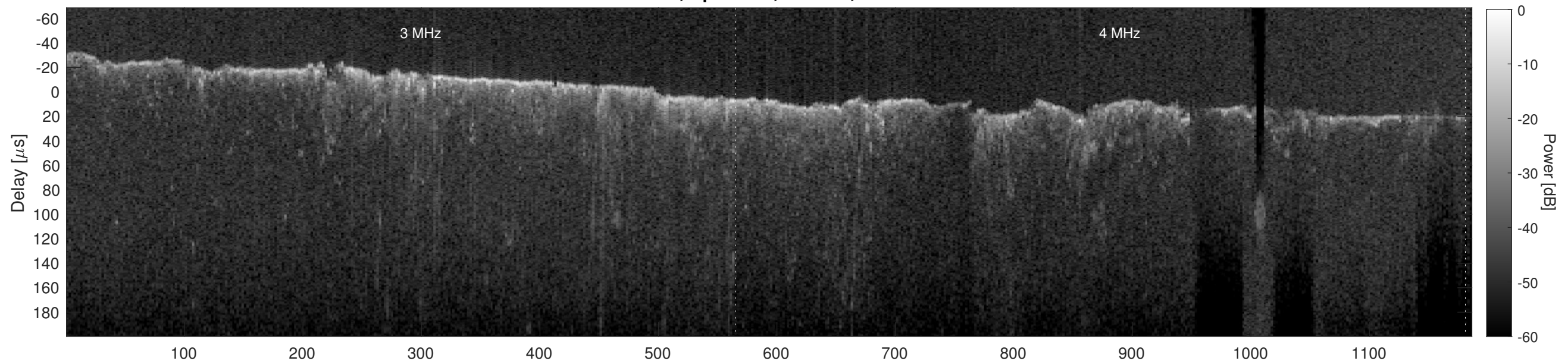
Orbit 8300, Cluttergram
