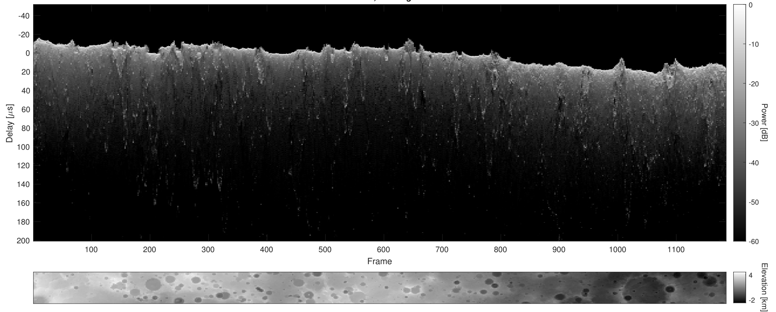
Orbit 8303, Cluttergram
