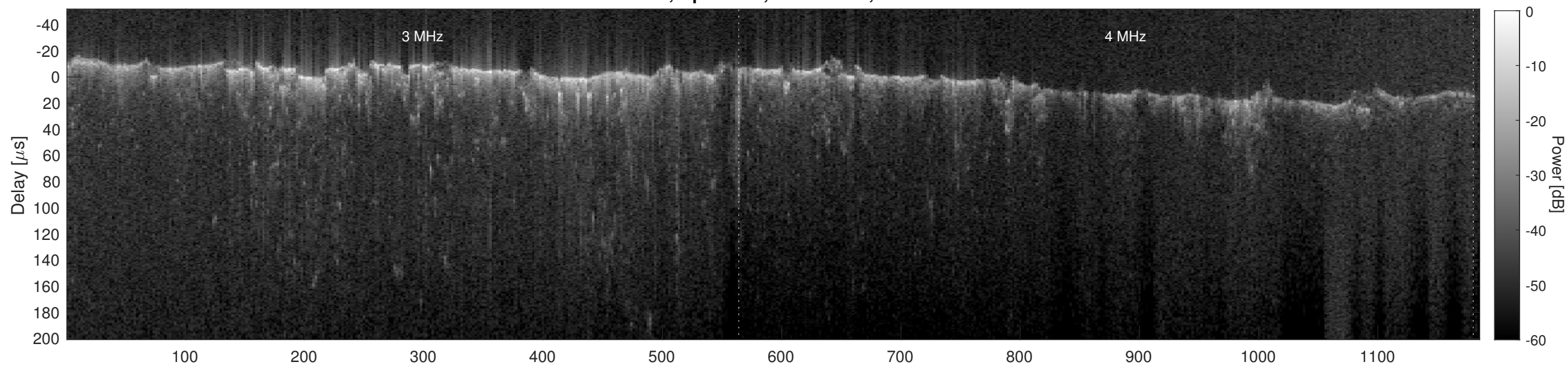
Orbit 8303, Cluttergram
