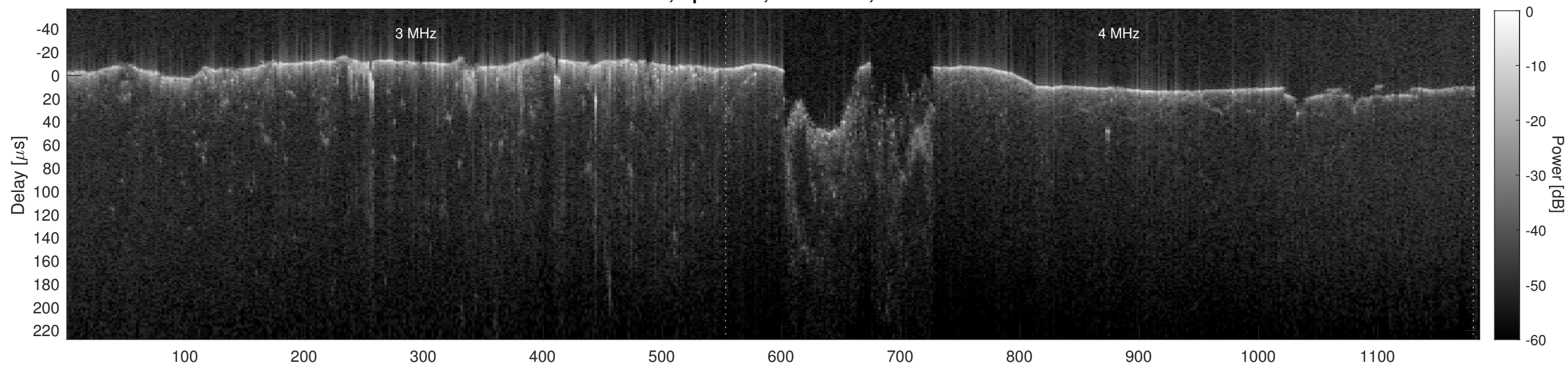
Orbit 8304, Cluttergram
