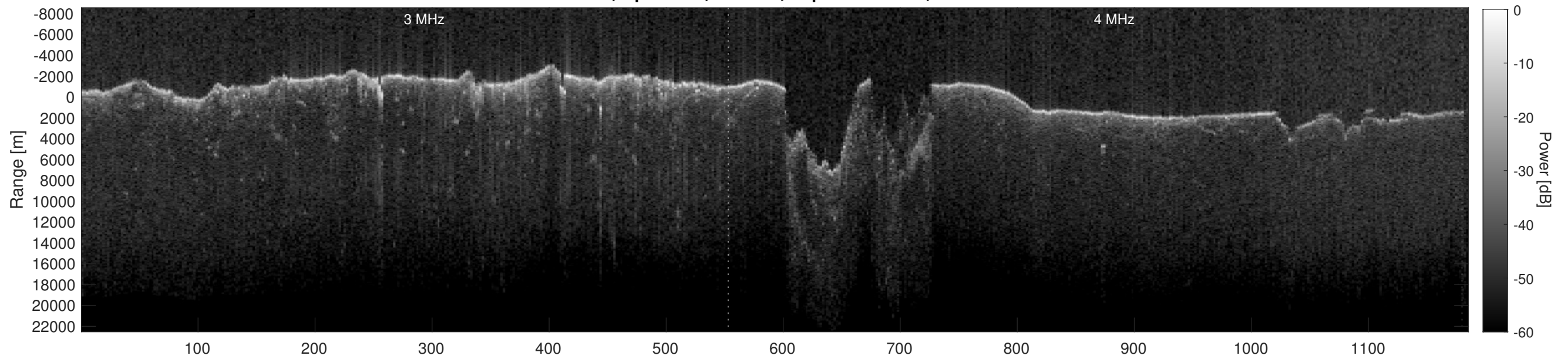
Orbit 8304, Depth-Corrected Cluttergram
