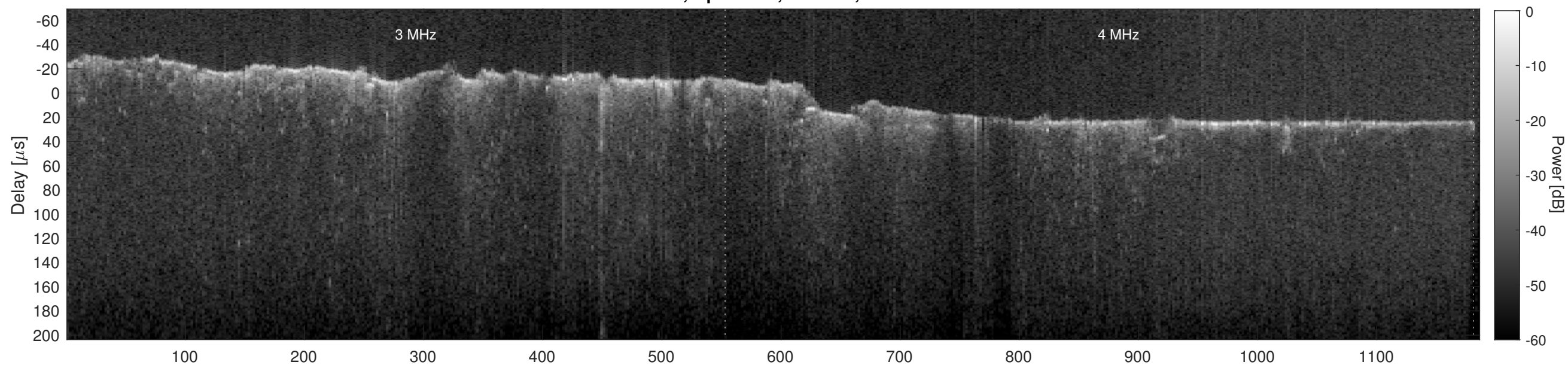
Orbit 8305, Cluttergram
