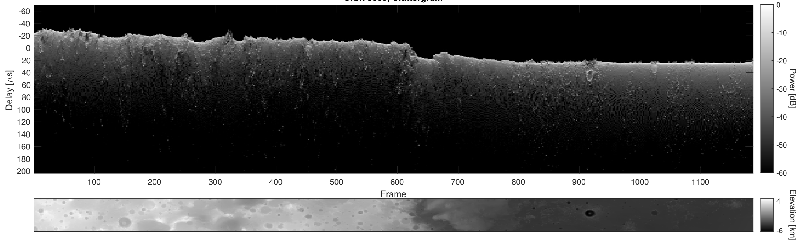
Orbit 8305, Cluttergram
